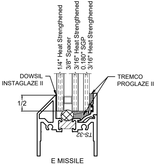
GLAZING DETAIL
