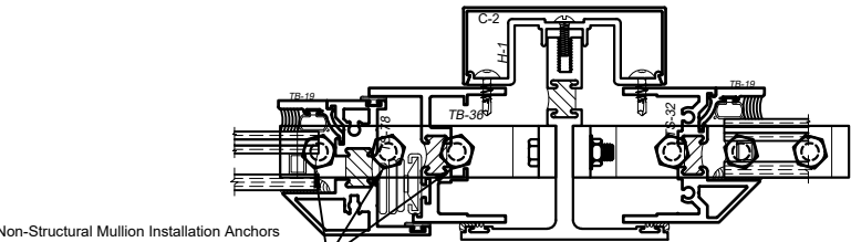
SECTION B: ANCH4 (SILL SIMILAR)
